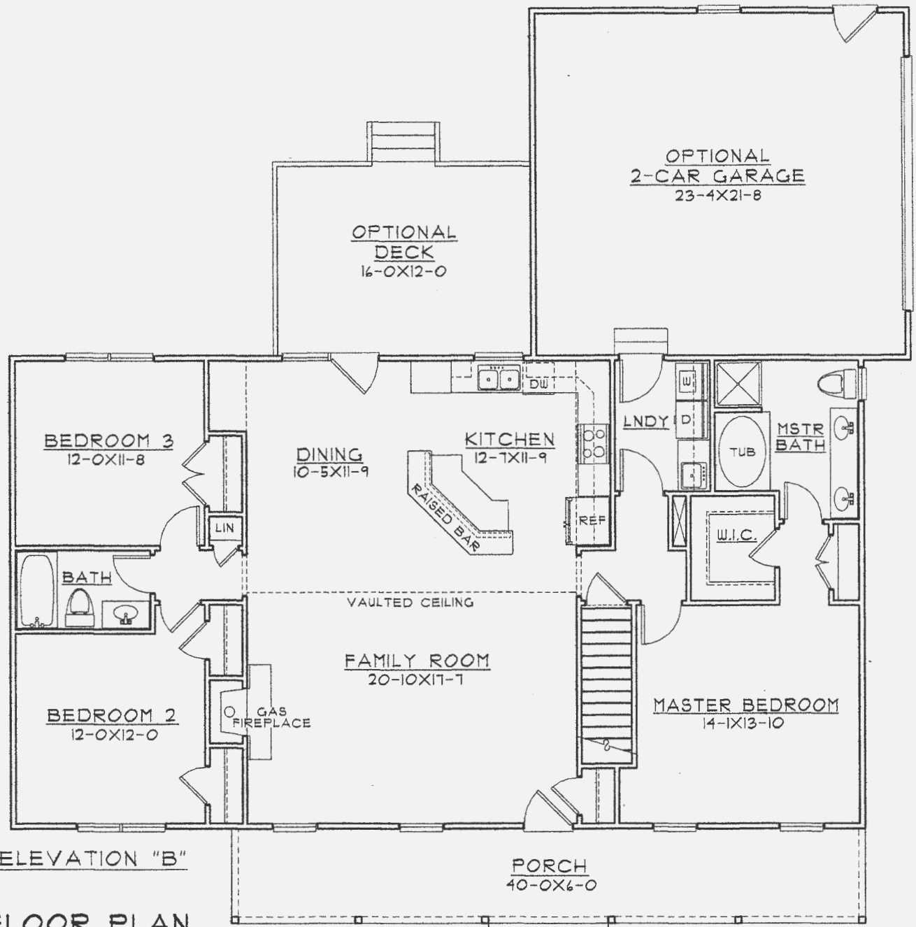
FIRST FLOOR PLAN 1620 SQ. FT.
