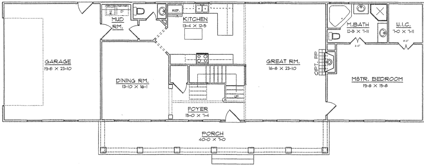
FIRST FLOOR PLAN - OPTION "B"
