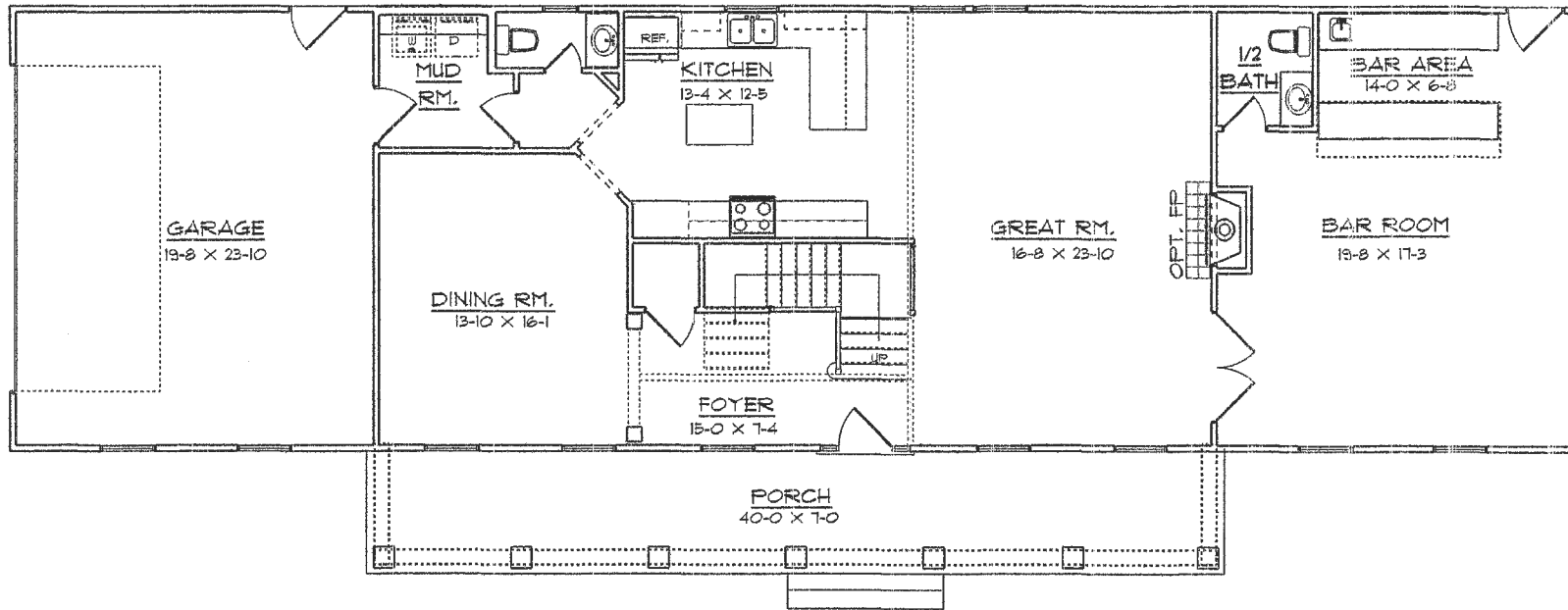
FIRST FLOOR PLAN - OPTION "A"
